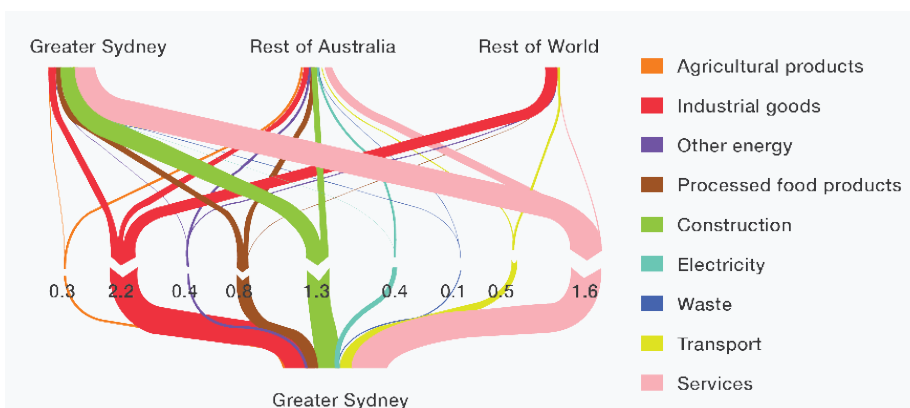
Figure 11: Distribution of GHG emissions across sectors and regions in 2040 for NEL scenario (t CO 2 eq).
