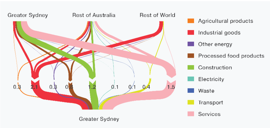
Figure 9: Distribution of GHG emissions across sectors and regions in 2040 for PRL scenario (t CO 2 eq).
